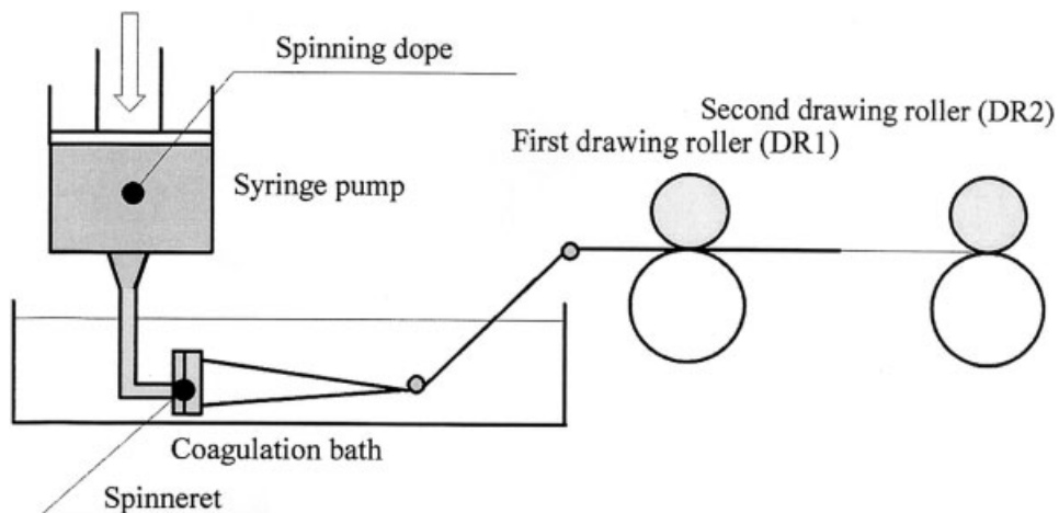
Figure 2 Schematic diagram of wet spinning apparatus.
